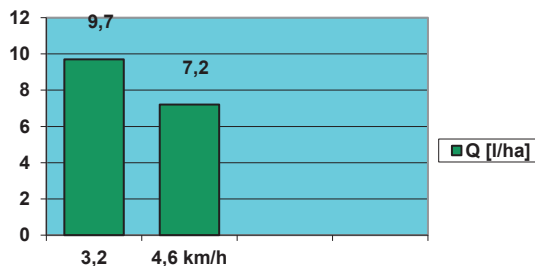
Fig. 3. Fuel consumption per unit area.
