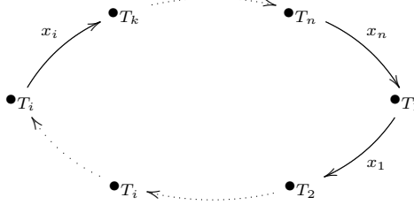
FIGURE 1. Cycle in G(h) of length n .
